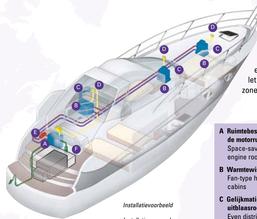
Installation example
